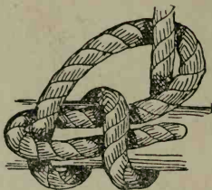
FIG. 50.—Studding-sail bend.
